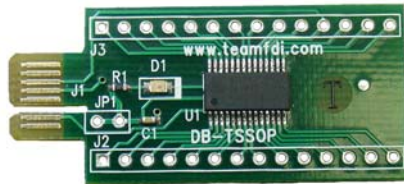
Board Dimensions 1.793" x 0.8"
