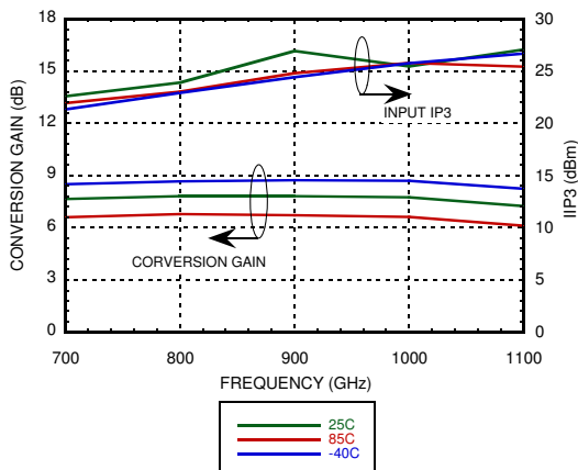
Figure-5a. IIP3 and Conversion Gain with matching for 900 MHz band VGATE=5.0 V, IF=100 MHz [1]
