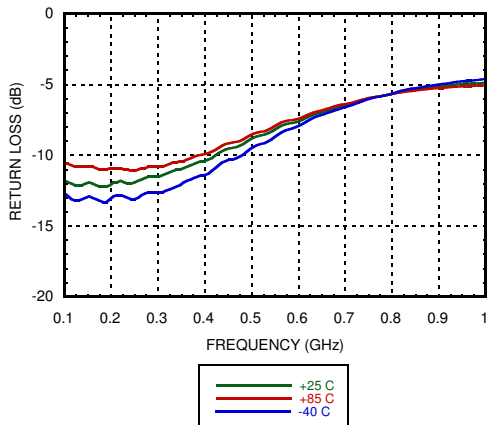
IF Output Return Loss @ VGATE=4.8V [1]
