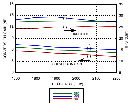
Figure-5b. IIP3 and Conversion Gain with matching for 1900 MHz band VGATE=4.8 V, IF=100 MHz [1]
