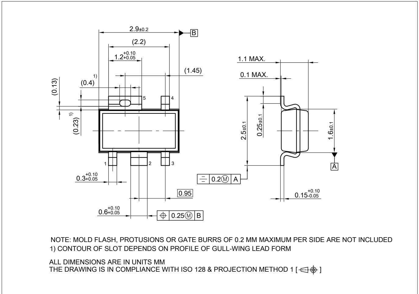
Figure 4 PG-SCT595-5
